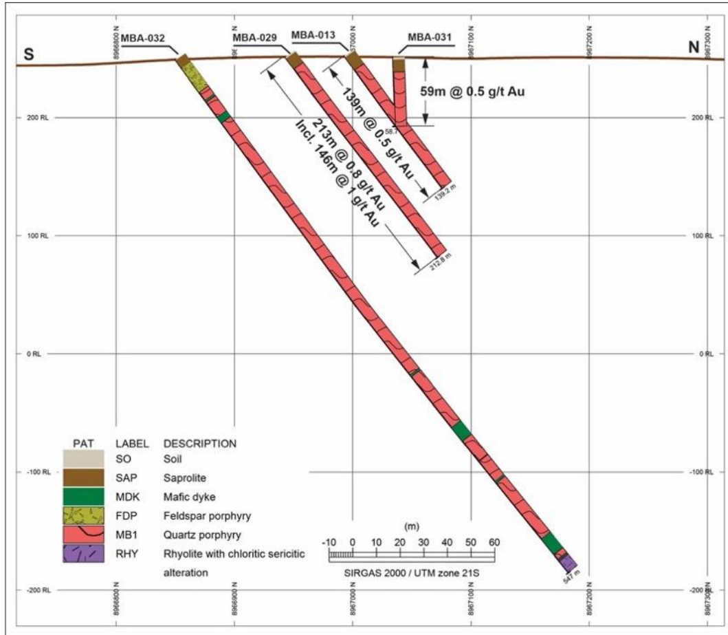
S-N cross-section through drill holes MBA-013, MBA-029, and MBA-032.
